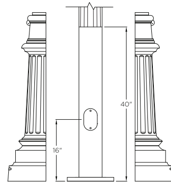
Split Base Detail with Shaft
