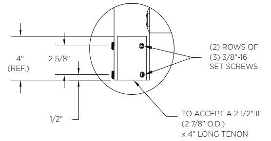
TENON DETAIL
