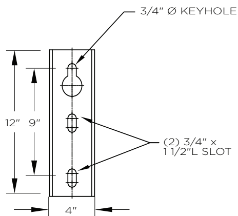
Side/Wall Mount Details
