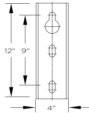
Side/Wall Mount Details 4" x 1 3/4" x 12"L
