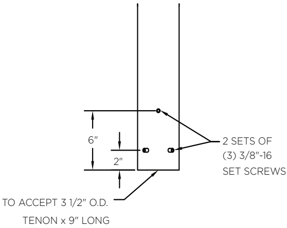
Tenon Mount Details
