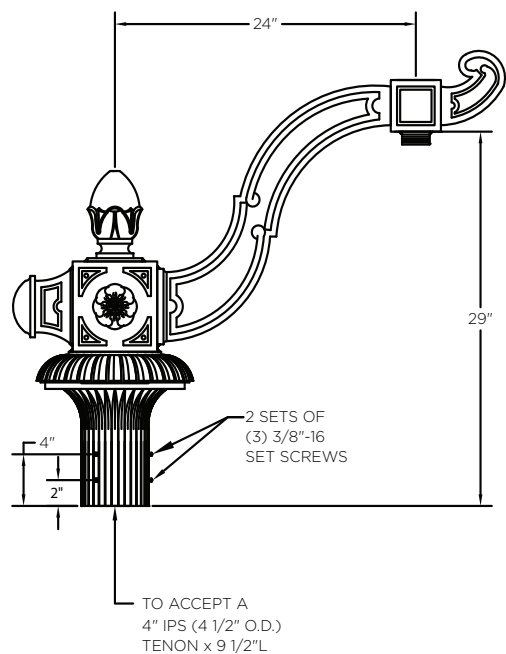
Tenon Mount Single Arm
