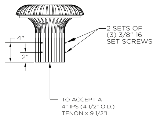
Tenon Mount Details
