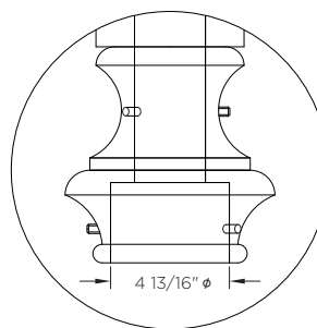
T1 Tenon Mount Details (4 1/2" Ø Pole Top)
