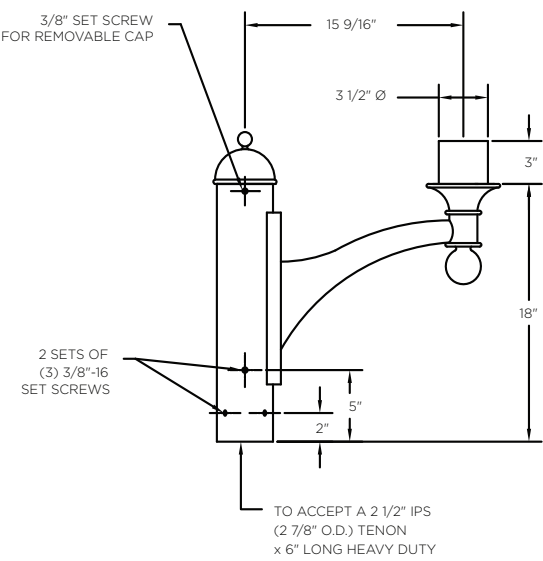
Tenon Mount Single Arm
