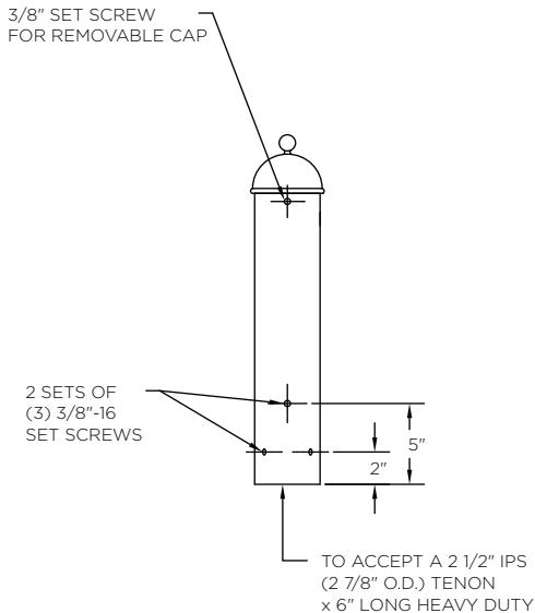
Tenon Mount Details
