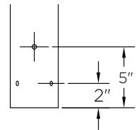
Tenon Mount Details To Accept a 2 1/2" IPS (2 7/8" O.D.) Tenon X 6" Long Heavy Duty
