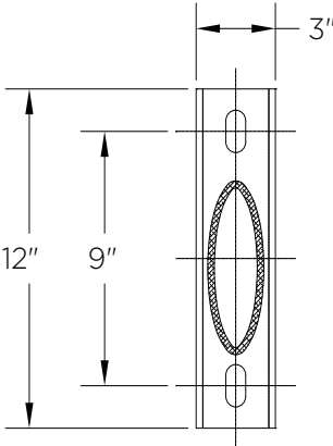
Side/Wall Mount Details
