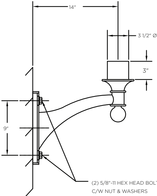
Wall Mount Single Arm
