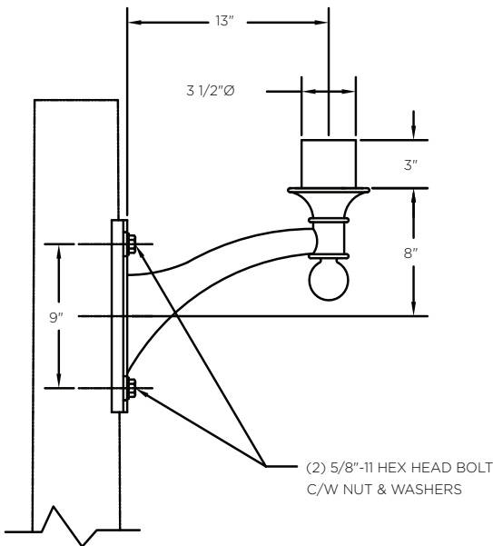
Side Mount Single Arm
