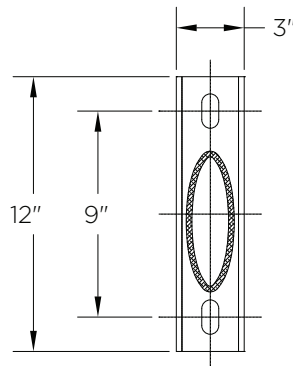
Side/Wall Mount Details 3" x 1 3/4" x 12"L
