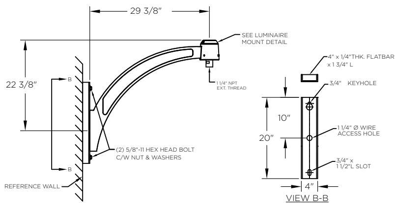
Wall Mount Single Arm
