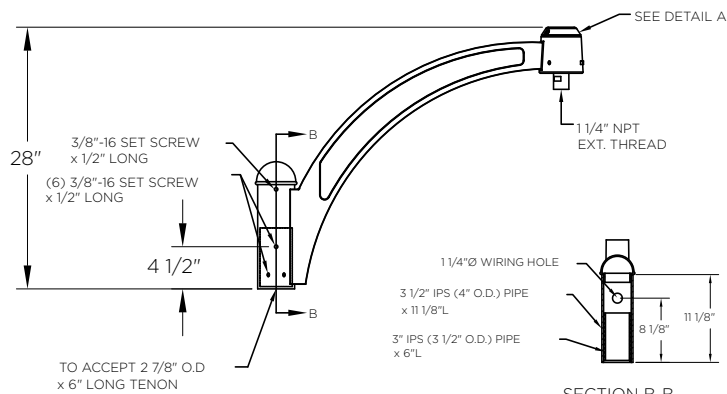
Tenon Mount Single Arm
