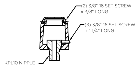
Luminaire Mounting Detail
