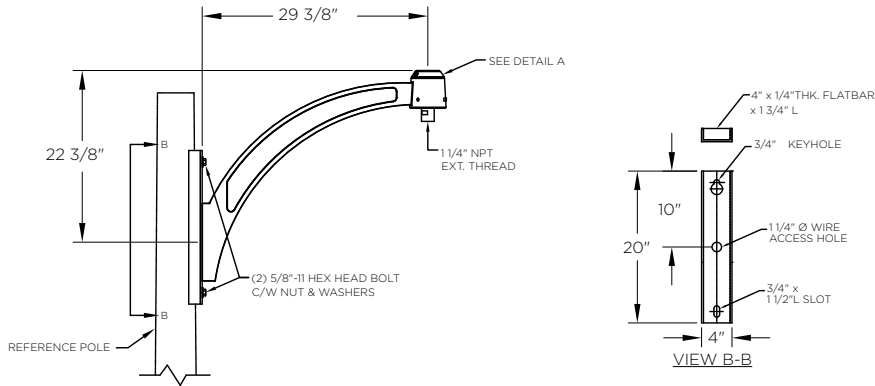
Side Mount Single Arm
