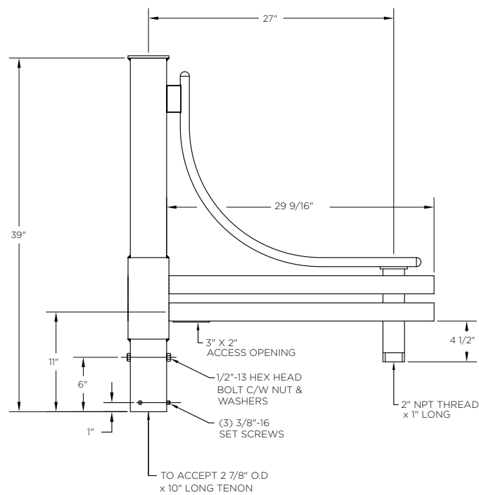
Tenon Mount Single Arm
