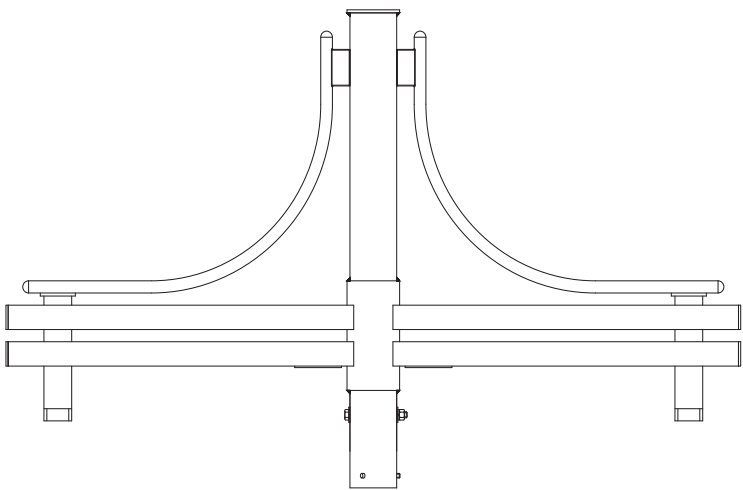
Tenon Mount Double Arm
