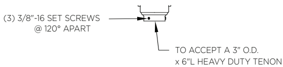
Tenon Mounting Details
