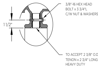
Tenon Mount
