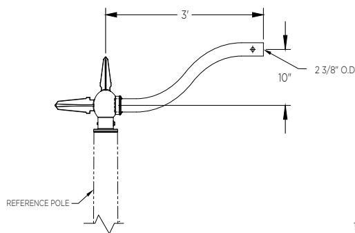
Tenon Mount
