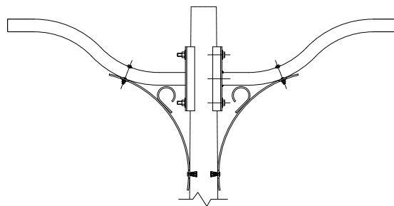
Side Mount Double Arm
