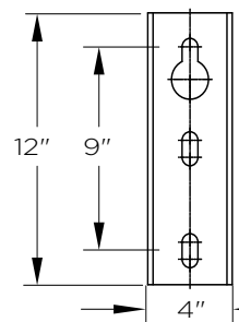
Side Mount Details 4" x 1 3/4" x 12"L
