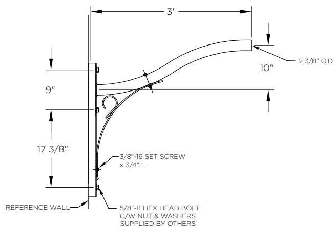
Wall Mount Single Arm
