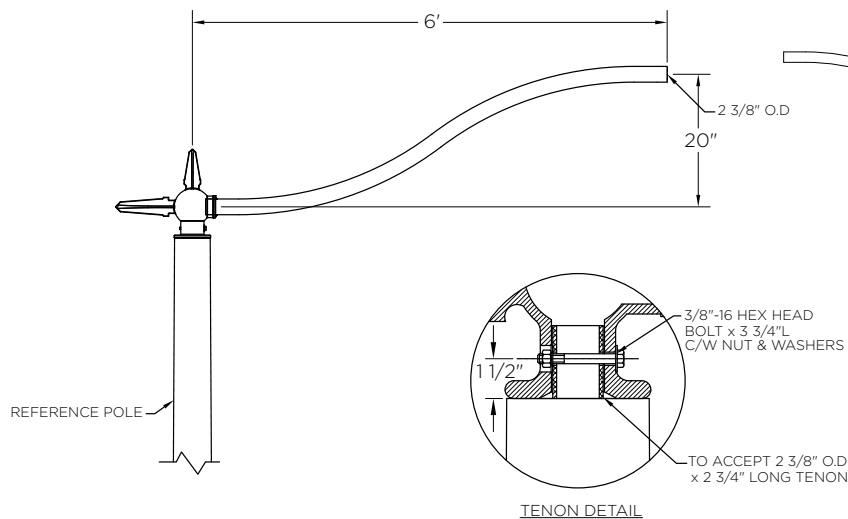
Tenon Mount Single Arm
