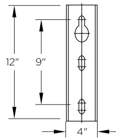
Side Mount Details 4" x 1 3/4" x 12"L
