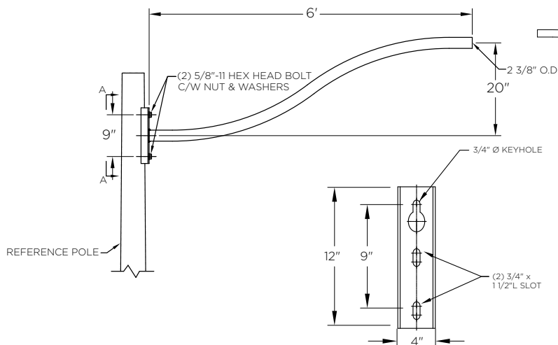
Side Mount Single Arm
