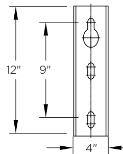
Side Mount Details 4" x 1 3/4" x 12"L
