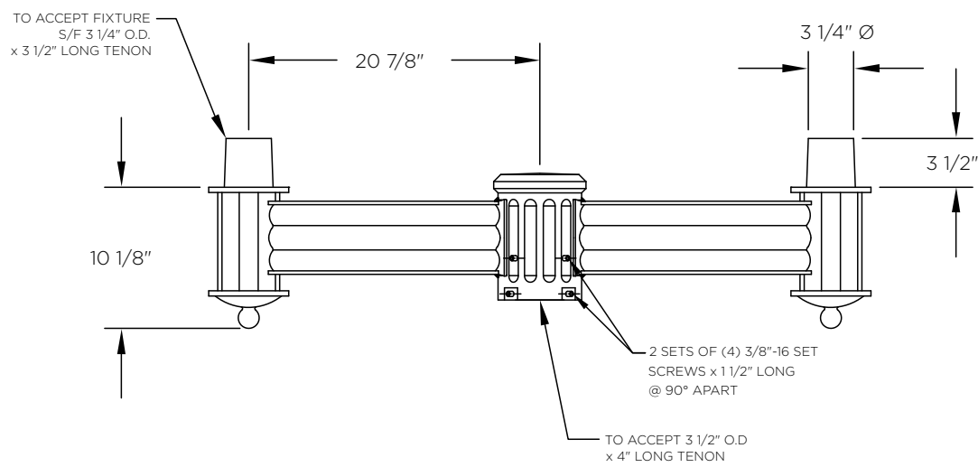
Tenon Mount Twin Arm
