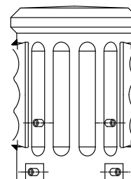
Tenon Mount Details TO ACCEPT 3 1/2" DIAMETER X 4"L TENON
