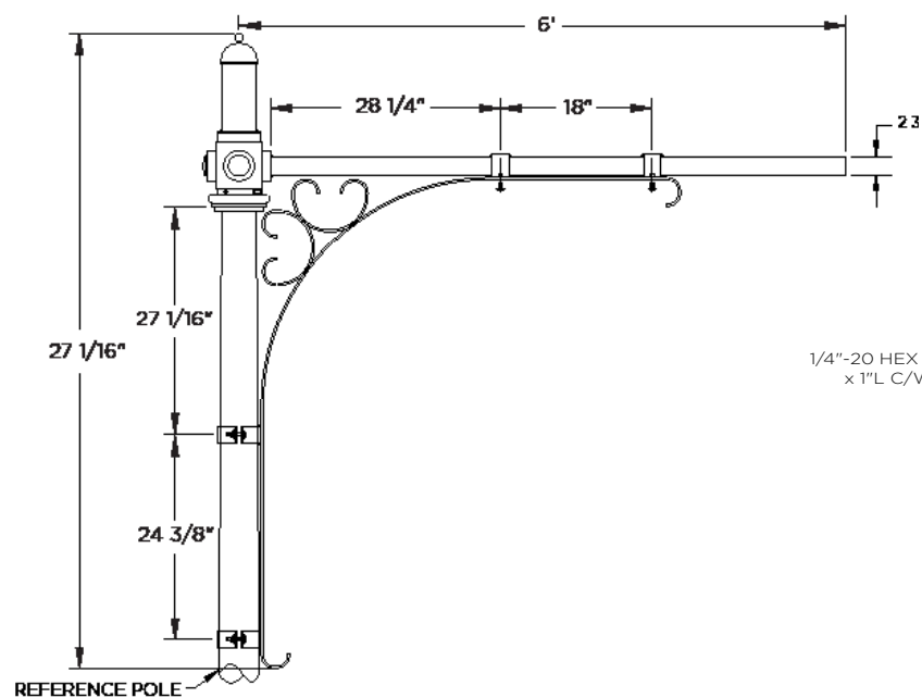
Tenon Mount Single Arm
