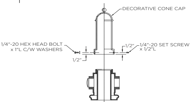
Decorative Cone Cap Details
