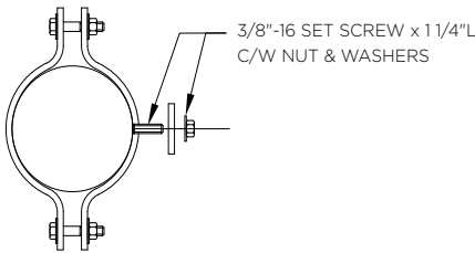
Clamp for Decorative Scroll Details (Bottom View)
