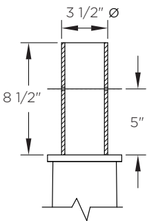
Tenon Mounting Details
