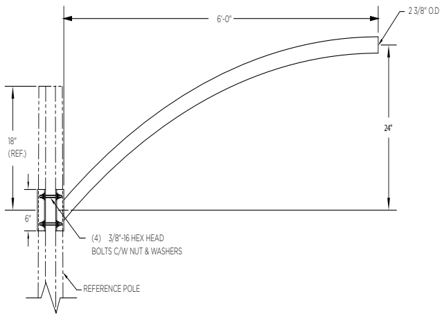
Side Mount Octagonal Single Arm
