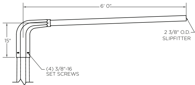
Top Octagonal Mount Single Arm
