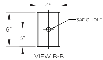
VIEW B-B
