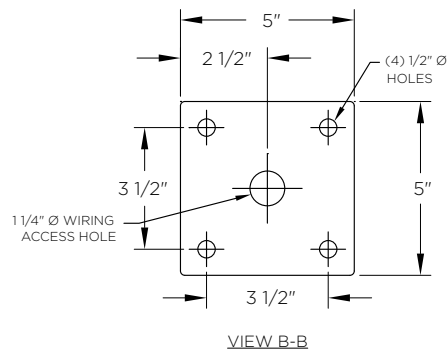
Luminaire Mounting Plate
