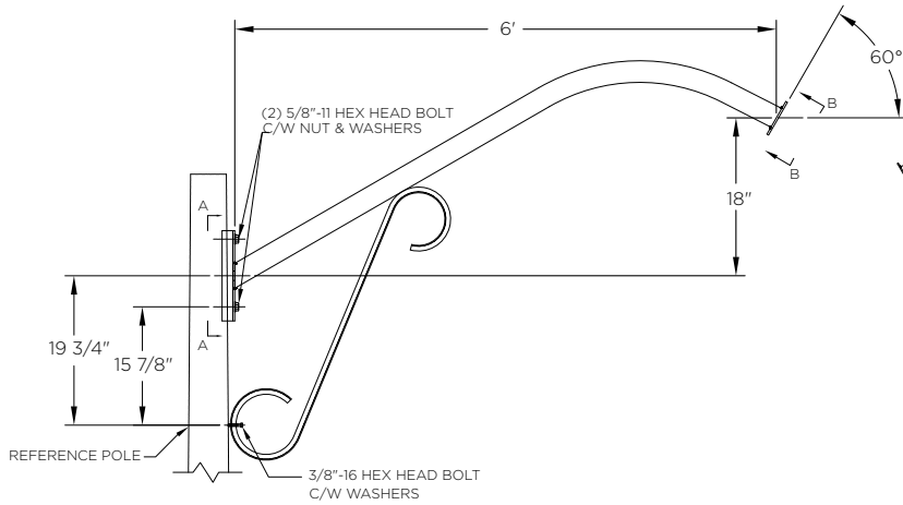
Side Mount Single Arm
