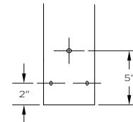
Tenon Mount Details To Accept A 2 1/2" IPS (2 7/8" O.D.) x 6" LG Heavy Duty Steel Tenon
