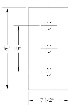
Wall Mount Details
