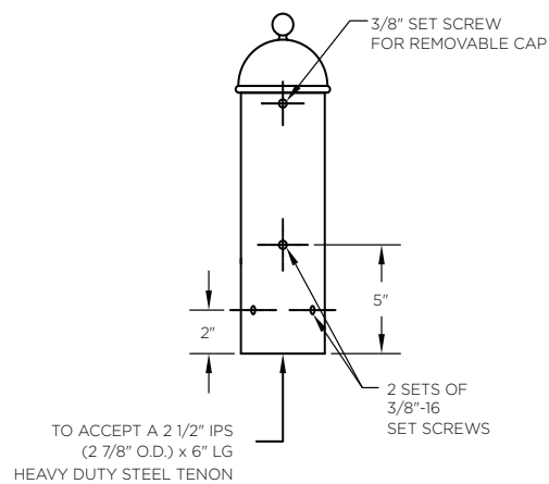
Tenon Mount Details
