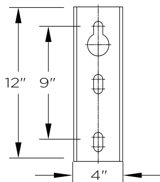
Side Mount Details
