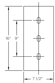
Wall Mount Details 4" x 1" x 12"L
