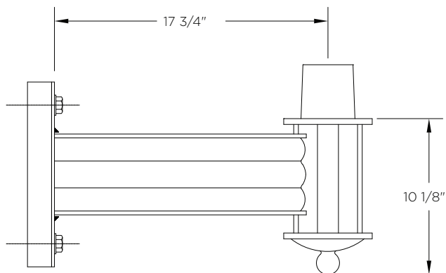
Side Mount Single Arm
