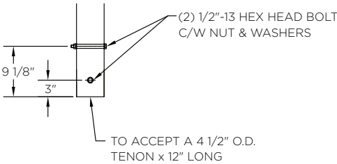
Tenon Mount Details
