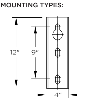
Side/Wall Mount Details 4" x 9" x 12"L
