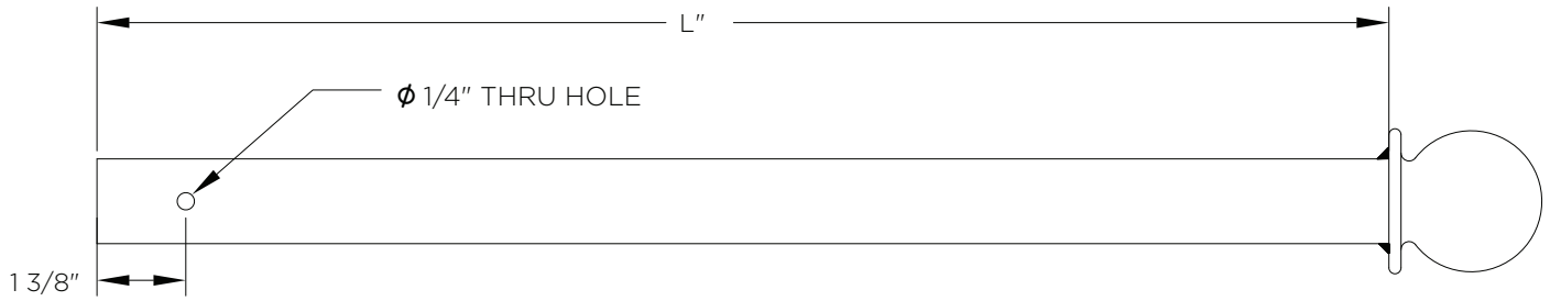
Single Banner Arm
