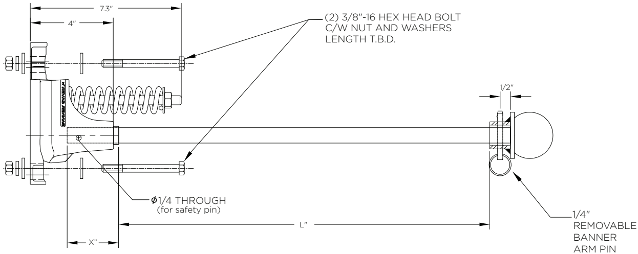
Single Banner Saver
