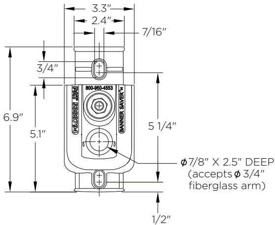
Mounting Details
