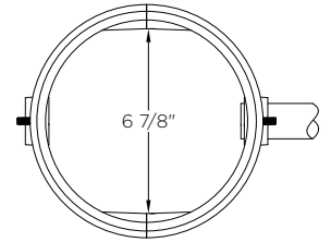
Cast Clamp-On (Large) (s/f 5 1/4" - 6 1/2" O.D. or FLAT/FLAT Pole)
