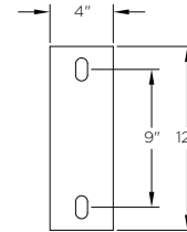
Side Channel
