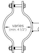
Fabricated Clamp-On (s/f varying shaft sizes - min. 4 1/2" O.D.)
