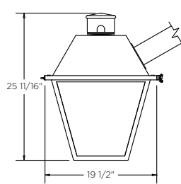
Side Mount
