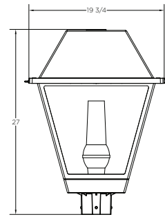
Aluminum Candle
