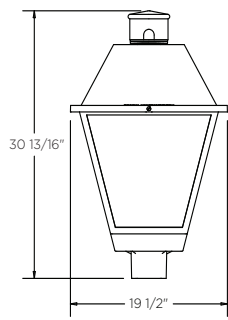
Post Top
